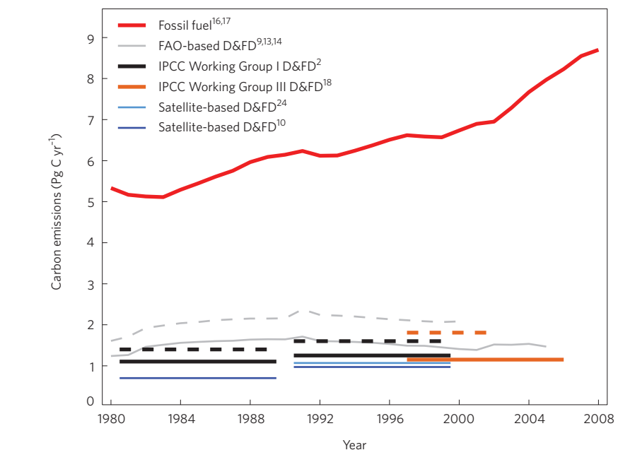
Figure 1 | Carbon emissions from deforestation and forest degradation (D&FD) and fossil fuel emissions for 1980 onwards. Updated datasets and approaches are depicted with a solid line, outdated ones with a dashed line. The often-held assumption that deforestation and forest degradation accounts for 20% of global anthropogenic CO 2 emissions is calculated using the average (dashed black line) of the deforestation surveys from the Food and Agricultural Organization (FAO; dashed grey line) and satellites in the 1990s (dark blue line), compared with average fossil fuel emissions estimates for the 1990s (red). Revised FAO-based emissions estimates (solid grey line) together with increased fossil fuel emissions substantially lower the relative contribution of deforestation and degradation to total anthropogenic emissions to about 12%. Dashed brown line indicates D&FD assessment used in IPCC Working Group III; solid brown line follows the same approach, but is based on updated carbon emissions from tropical forest fires used in this approach. Error bars are not shown, but the uncertainty in the deforestation figures is large, up to 50%. Peatland carbon emissions (0.30 Pg C yr -1 ) not included in emissions estimates.
