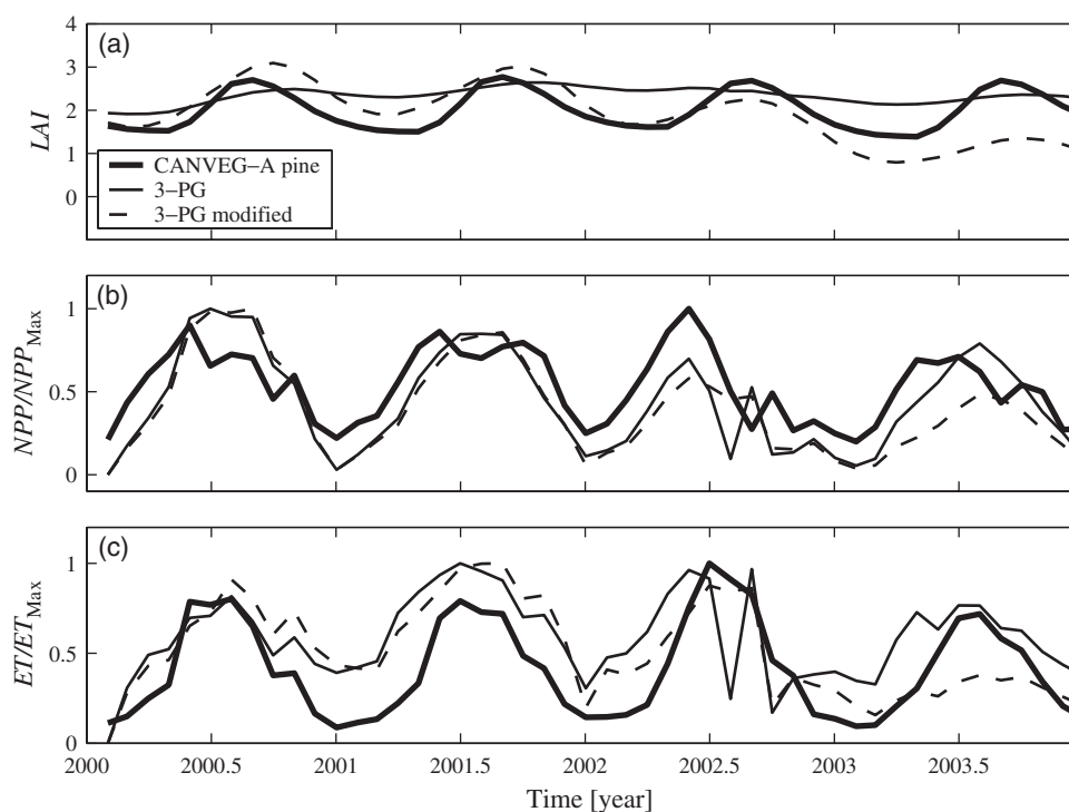
Fig. 1 Time series for pine leaf area index ( LAI ), normalized net primary production ( NPP ), and normalized evapotranspiration ( ET ) for the CANVEG with carbon allocation (CANVEG-A), the original physiological principles in predicting growth (3-PG), and 3-PG modified to include a new litterfall parameterization.
