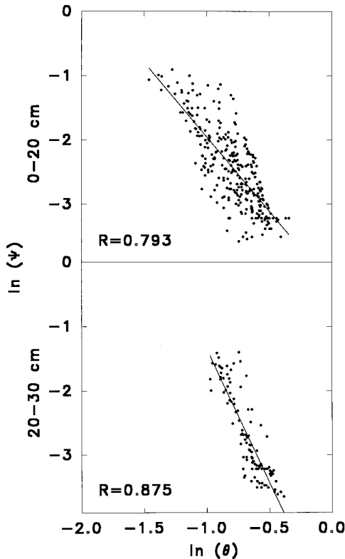
Figure 2. Determination of the soil water characteristic curve and the Clapp and Hornberger [1978] soil hydraulic parameters. The TDR and block resistance measurements, and the linear regression fit \ln |\Psi| = -b \ln (\theta/\theta_s) + \ln |\Psi_s| are shown for the 0–20 cm and 20–30 cm layers for all seven drying cycles.
