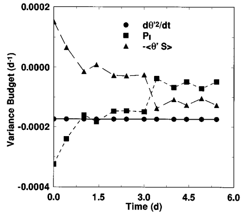
Figure 5b. The time evolution of the variance budget terms -2\langle\theta'S'\rangle (estimated as a residual in (9)), P_1 (estimated from (A9)), \partial\langle\theta'^2\rangle/\partial t (fitted to the \langle\theta'^2\rangle time TDR measurements) variance budget for the long drying period.
